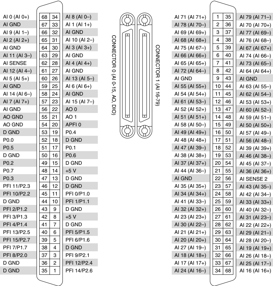
Figure 8. NI PXle-6345 Pinout
